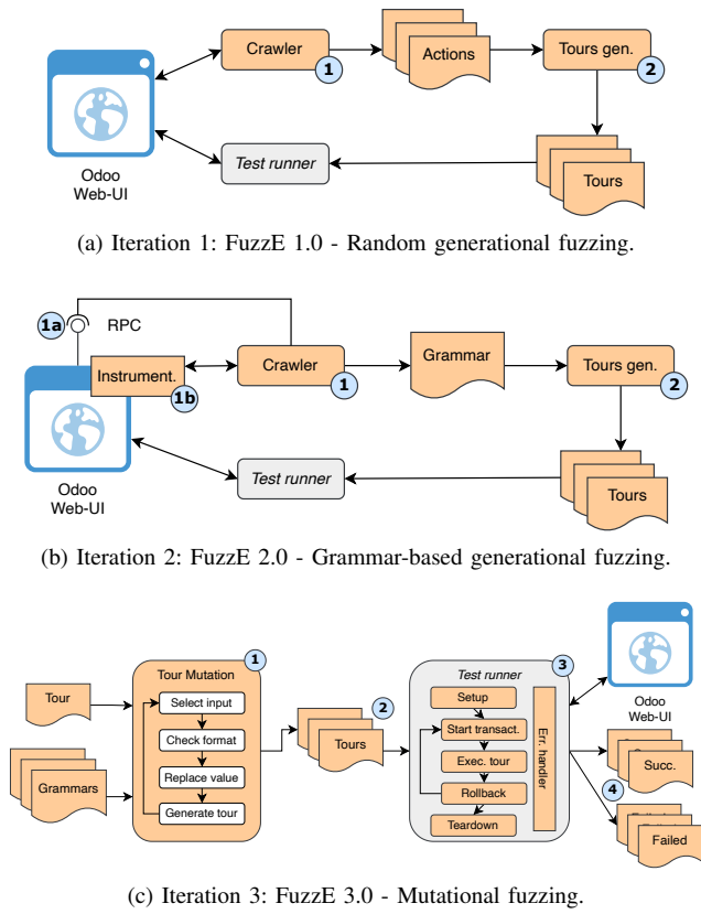
Fig. 1. FuzzE conceptual evolution over three iterations.
